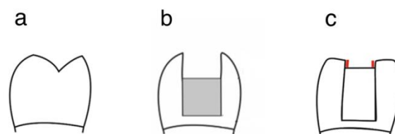
Figure 2. (a) Intact teeth, (b) cavity preparation in the composite group, (c) cavity preparation in the FRC group. Red lines represent the position of fiber ribbons
